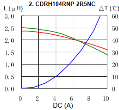
Saturation Current & Temperature Rise Graph — L (20°C) — L (105°C) — \Delta T
