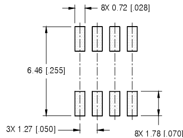
FOOTPRINT
